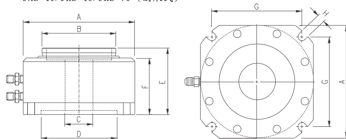
JAS-40/JHS-40/JHS-70 (副爪式)
