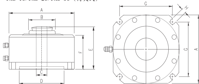
JAS-15/JAS-25/JAS-5C (筒夾式)
